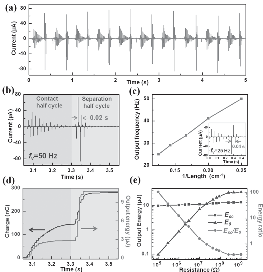
Figure 5. a) The output current curve with multiple cycles at a load resistance of 2 MΩ of the single-channel TEG-TENG with an output frequency of 50 Hz and a motion triggering frequency of 2 Hz. b) The magnification of the output current curve in a single cycle. c) The dependence of the output frequency on 1/L , and the inset shows the output current curve at a load resistance of 2 MΩ with an output frequency of 25 Hz. d) The curves of the absolute quantity of the flowed charges and the output energy in a single cycle. e) The dependences of E_{sc} , E_0 , and E_{sc}/E_0 on the load resistance.
